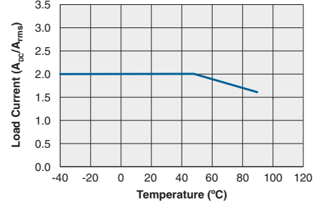
Typical Load Current vs. Temperature ( I_F=10\text{mA} )
