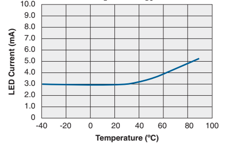
Typical I_F for Switch Operation vs. Temperature ( I_L=100\text{mA}_{DC} )
