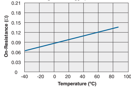
Typical On-Resistance vs. Temperature ( I_L=100\text{ mA}_{DC} , I_F=10\text{mA} )
